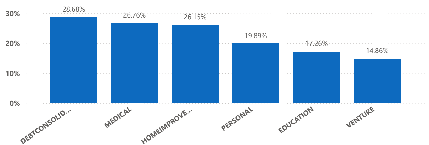
Default Rate by Loan Intent
